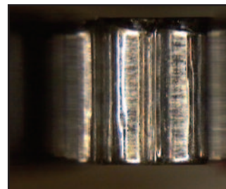
Unplated Crimper Surface after 60,000 Terminations. Note Significant buildup of material.
