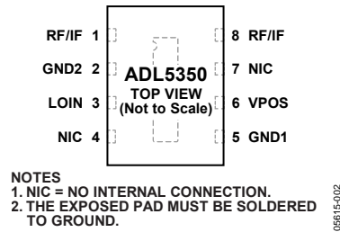
Figure 2. Pin Configuration
