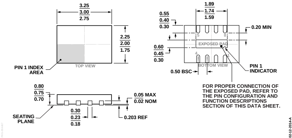
Figure 66. 8-Lead Lead Frame Chip Scale Package [LFCSP] 2 mm x 3 mm Body and 0.75 mm Package Height (CP-8-23) Dimensions shown in millimeters
