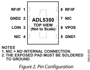
Figure 2. Pin Configuration
