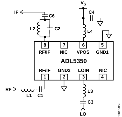
Figure 58. Reference Schematic
