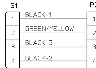
WIRING DIAGRAM
