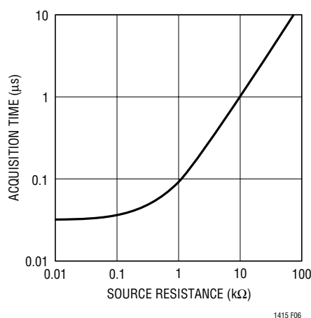
Figure 6. Acquisition Time vs Source Resistance
