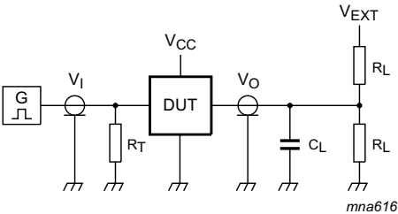
Measurement points are given in Table 10 . Definitions for test circuit: R_L = Load resistance. C_L = Load capacitance including jig and probe capacitance. R_T = Termination resistance should be equal to output impedance Z_o of the pulse generator. V_{EXT} = External voltage for measuring switching times.
