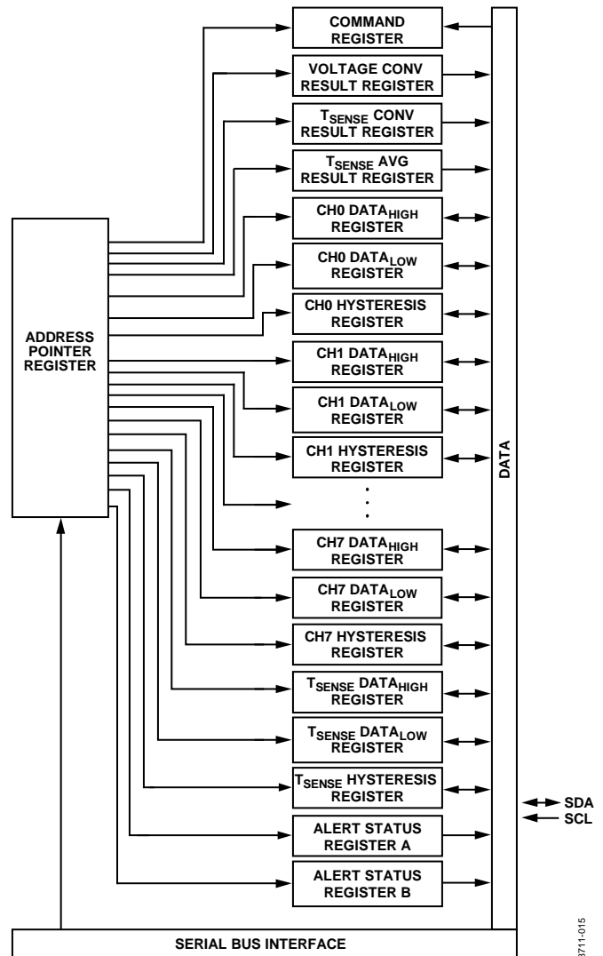
Figure 23. AD7291 Register Structure
