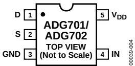
Figure 4. 5-Lead SOT-23
