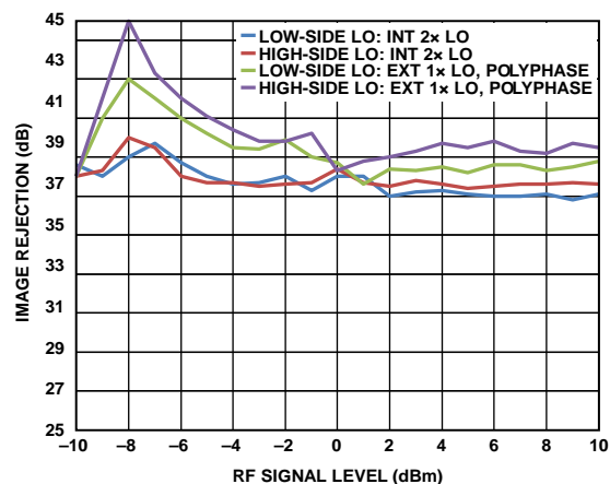
Figure 51. Image Rejection vs. RF Signal Level, IF = 200 MHz, for High-Side LO Injection f_{LO} = 2000 MHz and f_{IF} = 1800 MHz and Vice Versa for Low-Side Injection
