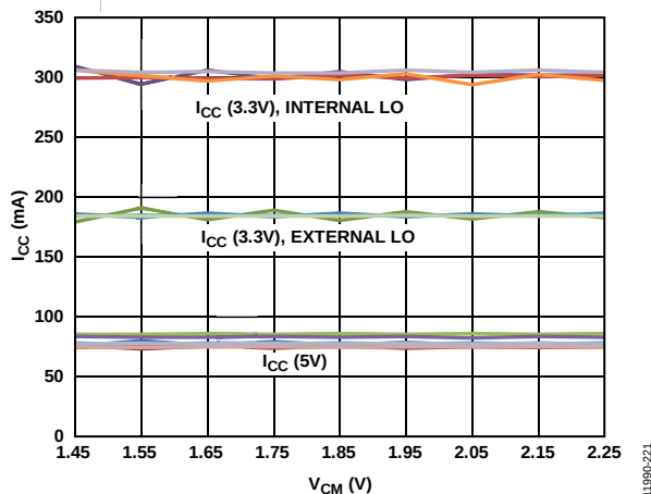
Figure 17. Current Consumption ( I_{CC} ) vs. Common-Mode Voltage ( V_{CM} ), Internal and External LO, f_{RF} = 900 MHz, f_{RF} = 1900 MHz, f_{RF} = 2100 MHz, f_{RF} = 2100 MHz, and f_{RF} = 2650 MHz
