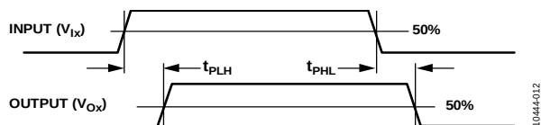
Figure 12. Propagation Delay Parameters
