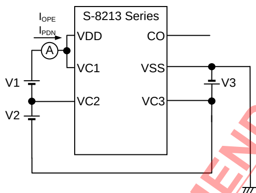
Figure 8 Test Circuit 3
