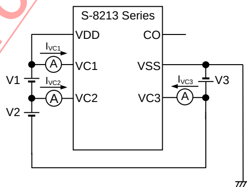
Figure 9 Test Circuit 4
