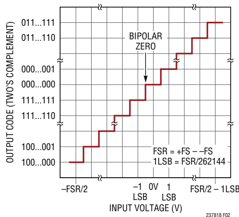
Figure 2. LTC2378-18 Transfer Function
