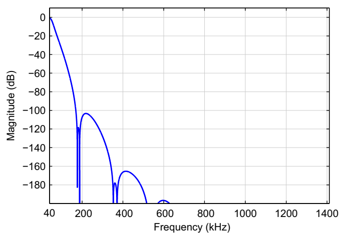
Figure 9-66. Stopband Attenuation
