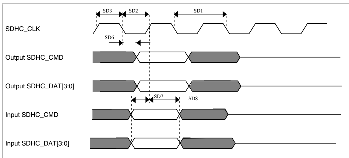
Figure 20. uSDHC timing
