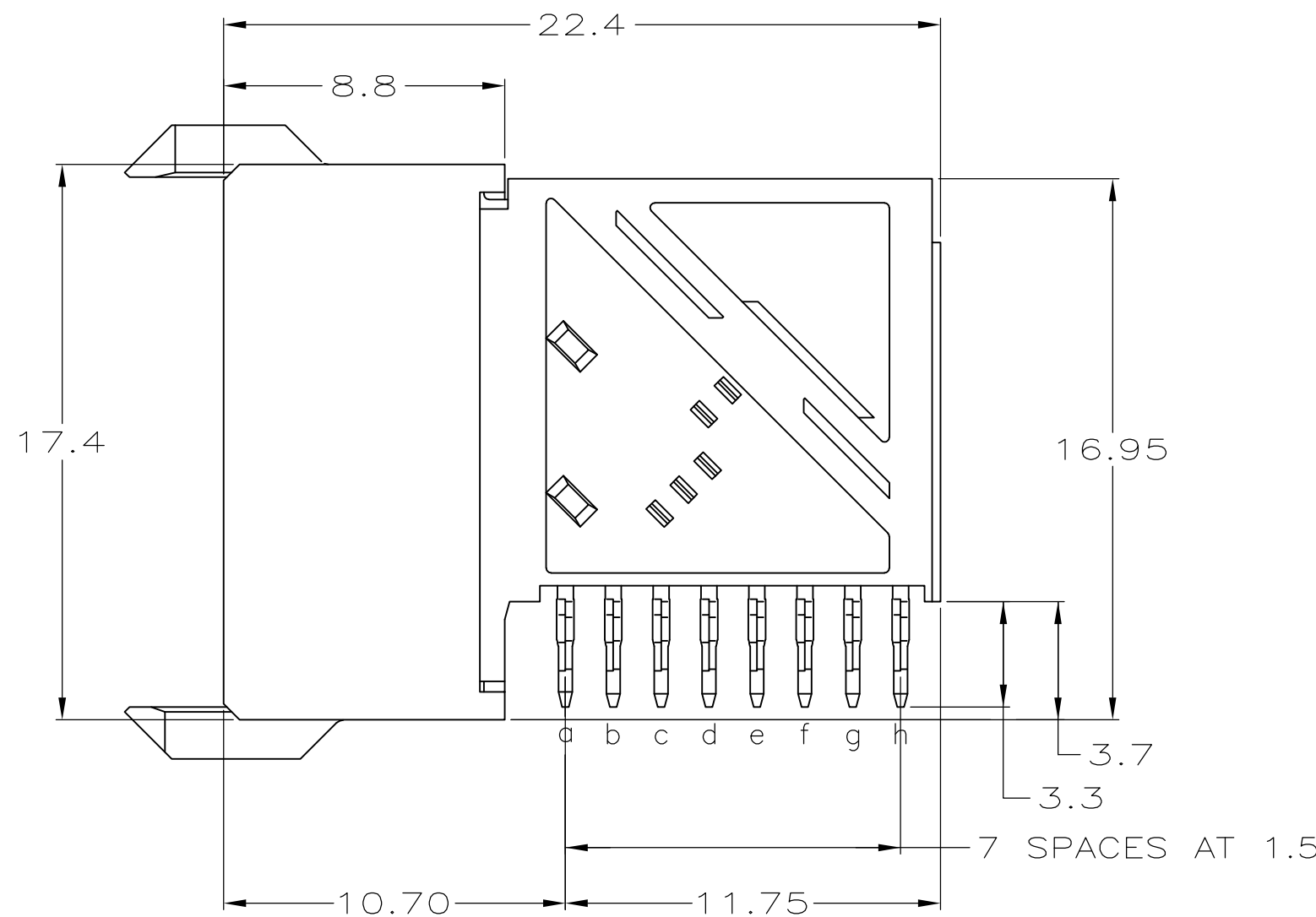
SECTION W-W
