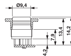
Dimensioned drawing
