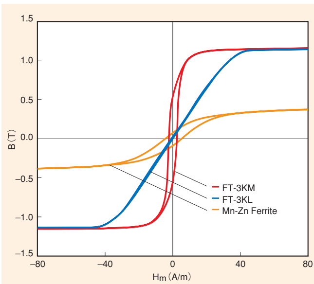
Figure 54. DC-BH Curves
