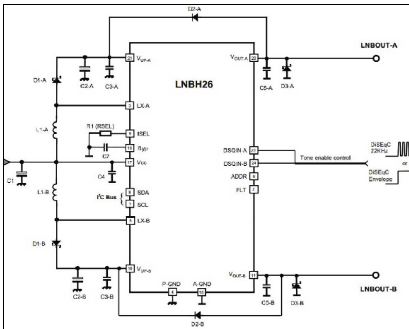
Figure 1: STEVAL-CBL012V1 schematic
