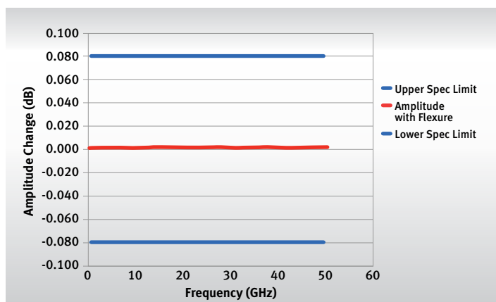
FIGURE 3: TYPICAL AMPLITUDE STABILITY WITH FLEXURE 1
