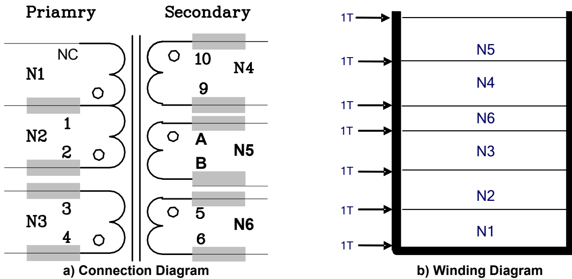
Figure 12: Transformer Structure
