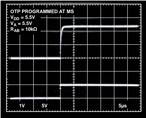
Figure 26. Power-Up Settling Time After Fuses Blown
