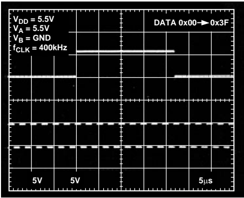
Figure 24. Large Settling Time
