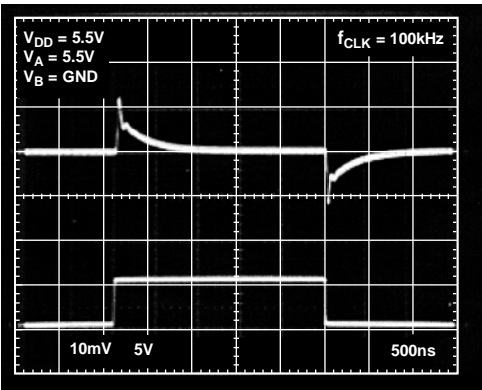
Figure 23. Digital Feedthrough
