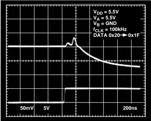
Figure 25. Midscale Glitch Energy
