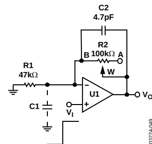
Figure 49. Typical Noninverting Gain Amplifier
