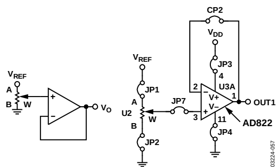
Figure 54. One Possible Configuration— Programmable Voltage Reference
