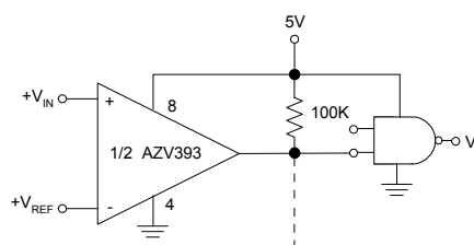
Figure 25. Driving CMOS
