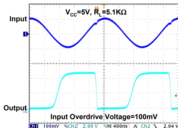
Figure 23. 500kHz Response
