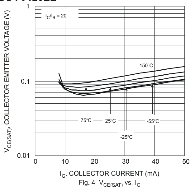
Fig. 4 V_{CE(SAT)} vs. I_C
