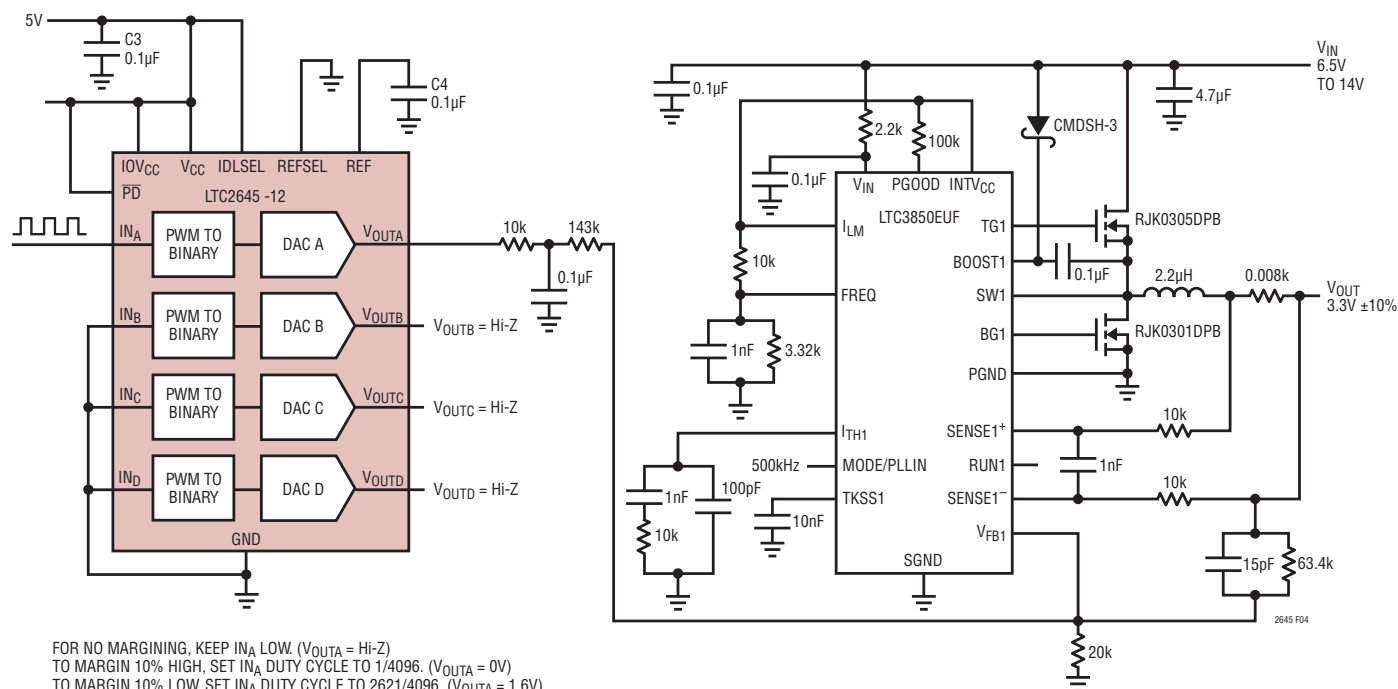
Figure 4. Voltage Margining Application with LTC3850 (3.3V \pm 10\% )
