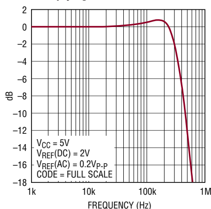
Multiplying Bandwidth
