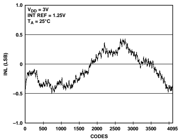
Figure 21. INL AD5628-1
