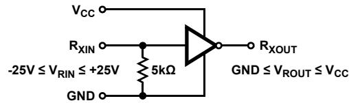
Figure 6. Inverting Receiver Connections
