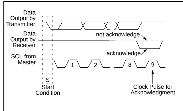
FIGURE 11-11: SLAVE-RECEIVER ACKNOWLEDGE
