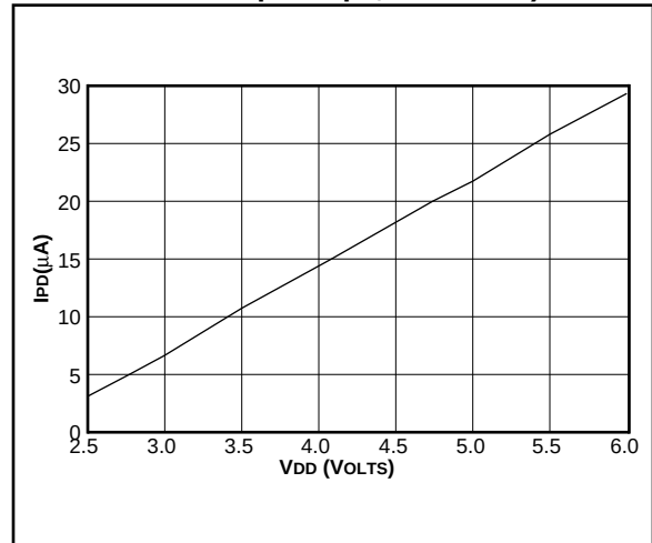
FIGURE 18-13: MAXIMUM I_{PD} vs. TIMER1 ENABLED (32 kHz, RC0/RC1 = 33 \text{ pF}/33 \text{ pF} , 85°C TO -40°C, RC MODE)
