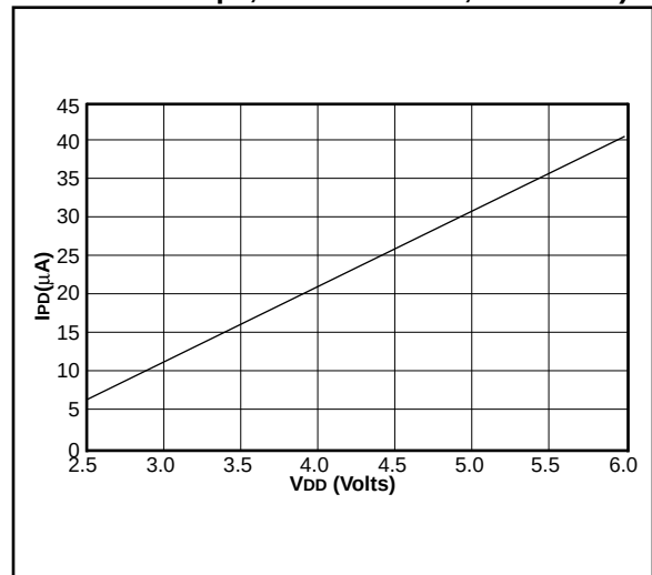
FIGURE 18-13: MAXIMUM I_{PD} vs. TIMER1 ENABLED (32 kHz, RC0/RC1 = 33 \text{ pF}/33 \text{ pF} , 85°C TO -40°C, RC MODE)
