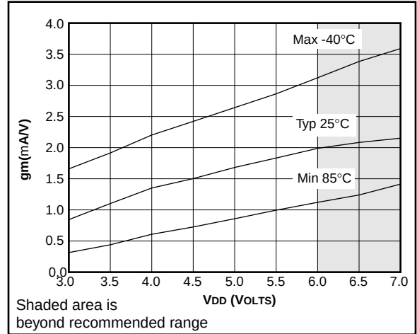
FIGURE 18-21: TRANSCONDUCTANCE(gm) OF LP OSCILLATOR vs. VDD
