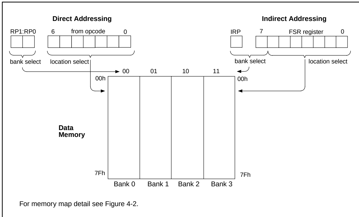
FIGURE 4-10: DIRECT/INDIRECT ADDRESSING
