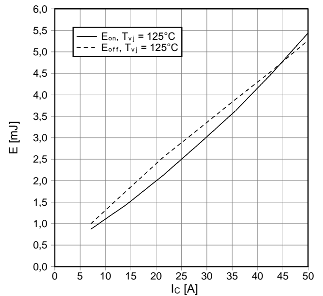
Schaltverluste IGBT-Wechselr. (typisch) switching losses IGBT-inverter (typical) E_{on} = f(I_c), E_{off} = f(I_c) V_{GE} = \pm 15\text{ V}, R_{Gon} = 36\ \Omega, R_{Goff} = 36\ \Omega, V_{CE} = 600\text{ V}
