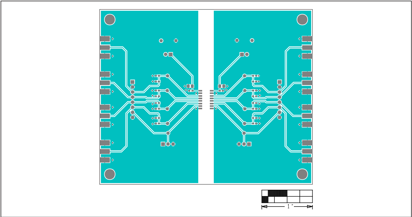
MAX14430–MAX14432 EV Kit—Bottom Silkscreen
