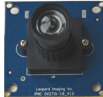
LI-CAM-OV2715-1.8 Camera Module
