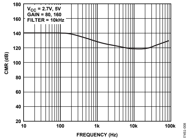
Figure 8. Common-Mode Rejection (CMR) vs. Frequency
