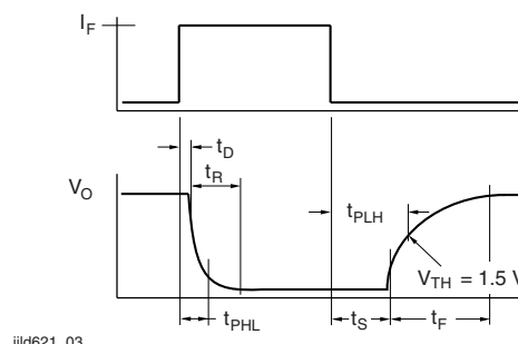
Fig. 3 - Saturated Switching Timing
