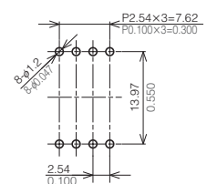
Recommended PC board pattern (BOTTOM VIEW)
