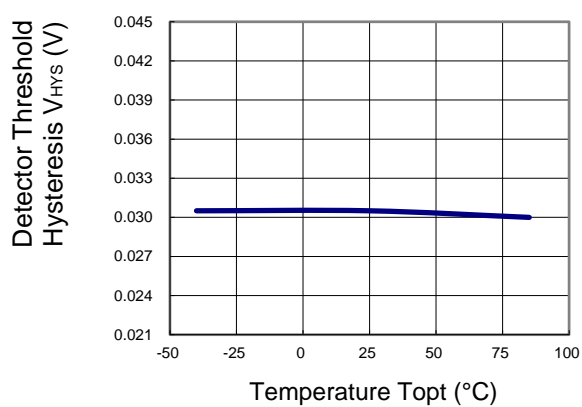
R3118x06xA/C ( V_{DD}=5.3\text{V} )
