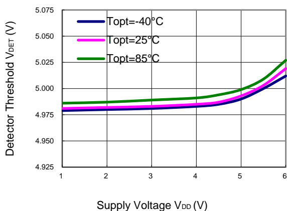
R3118x50xA/C
