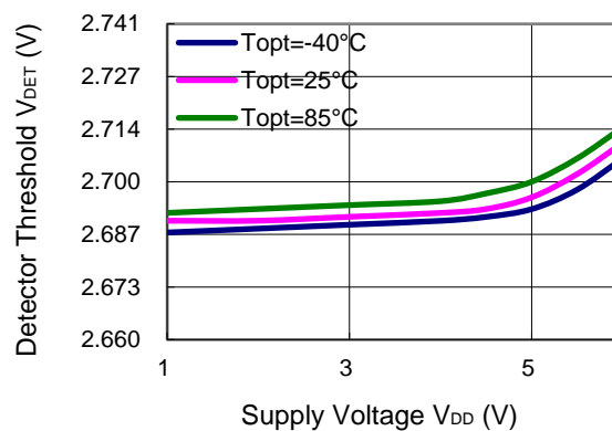
R3118x27xA/C
