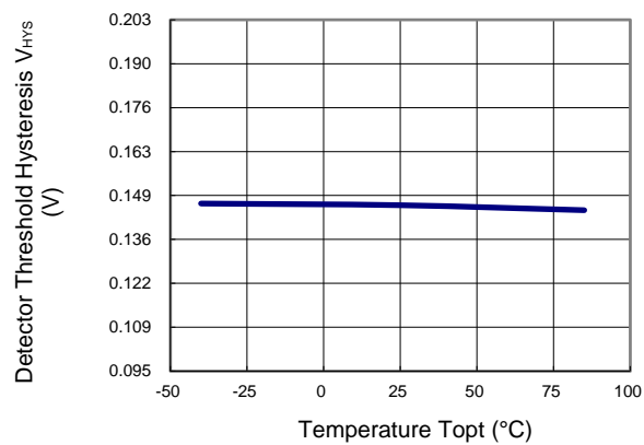
R3118x27xA/C ( V_{DD}=5.3\text{V} )
