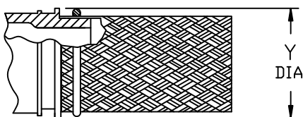
TINEL-LOCK TERMINATION
