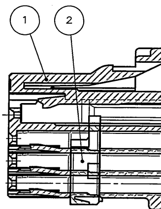
SECT. A-A
