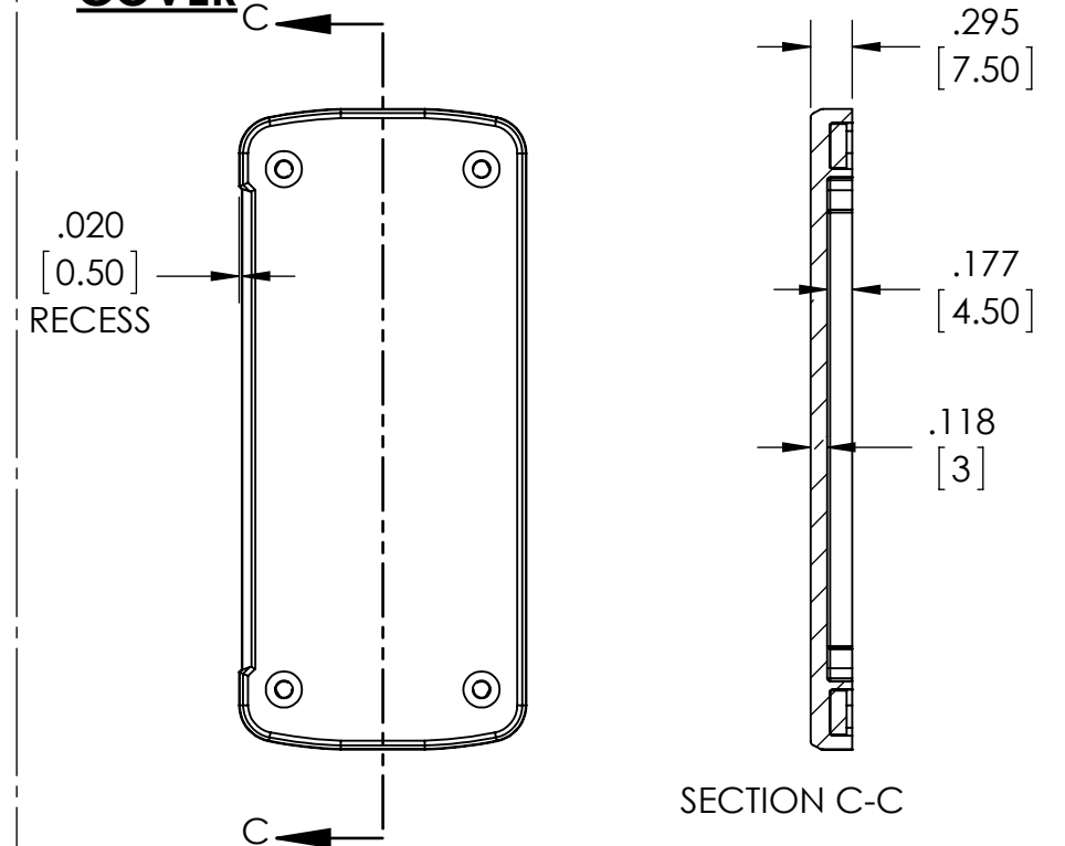
PLASTIC COVER
