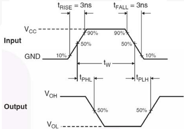
Figure 5. AC Waveforms
