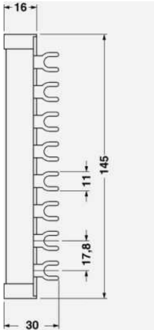
Dimensioned drawing
