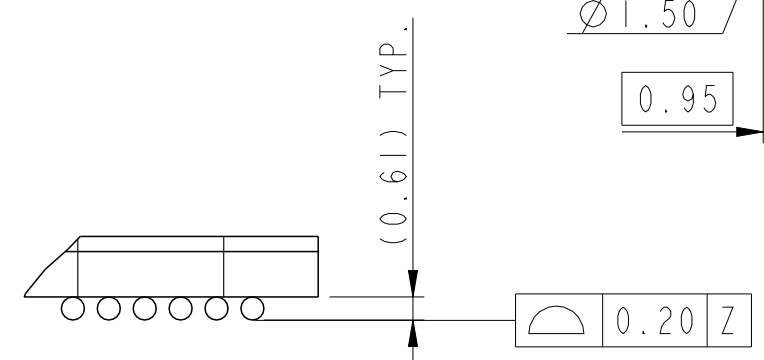
DETAIL B SCALE 5:1
