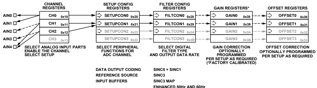
Figure 52. Mixed Differential and Single-Ended Configuration Using Multiple Shared Setups
