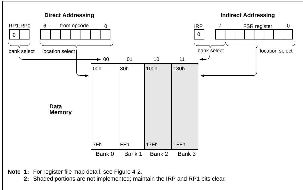
FIGURE 4-4: DIRECT/INDIRECT ADDRESSING
