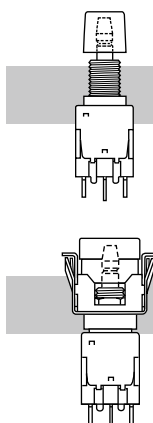
Snap-in Mount
