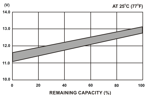
OPEN CIRCUIT VOLTAGE VS REMAINING CAPACITY
