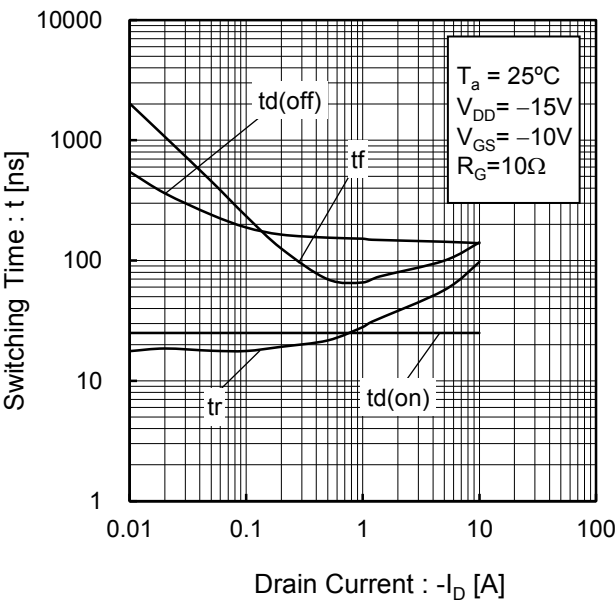
Fig.21 Switching Characteristics
